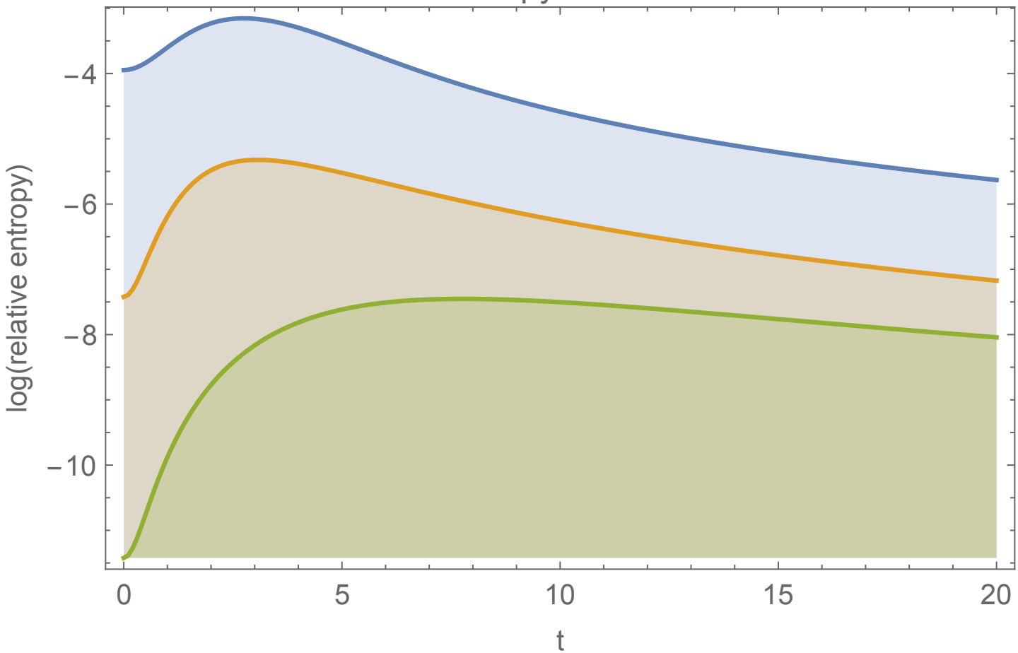
Relative entropy w.r.t. the normal
